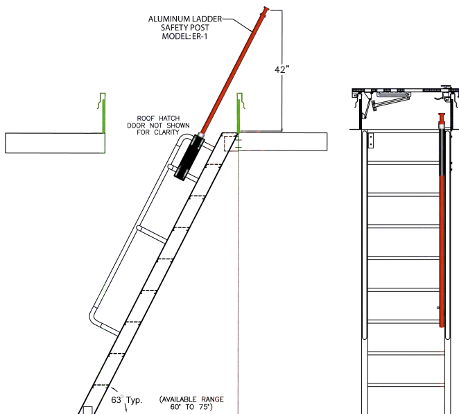
ALUMINUM SHIPS LADDER w/ EXTEND-A-RAIL TO ROOF HATCH
